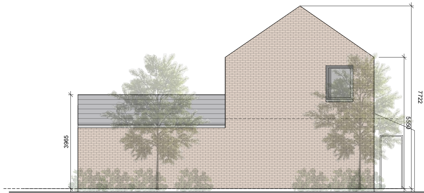
GABLE ELEVATION
